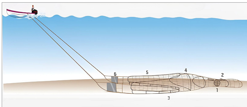
Figure 19. Chalut RS-INP-MX
