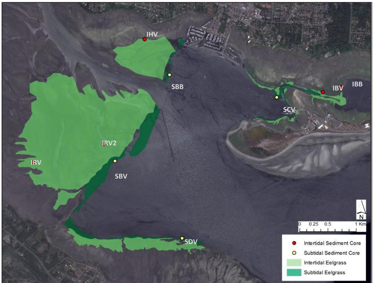
Figure 30. K'ómoks Estuary eelgrass bed area coverage showing core locations. Copyright 2015 by Comox Valley Project Watershed.
