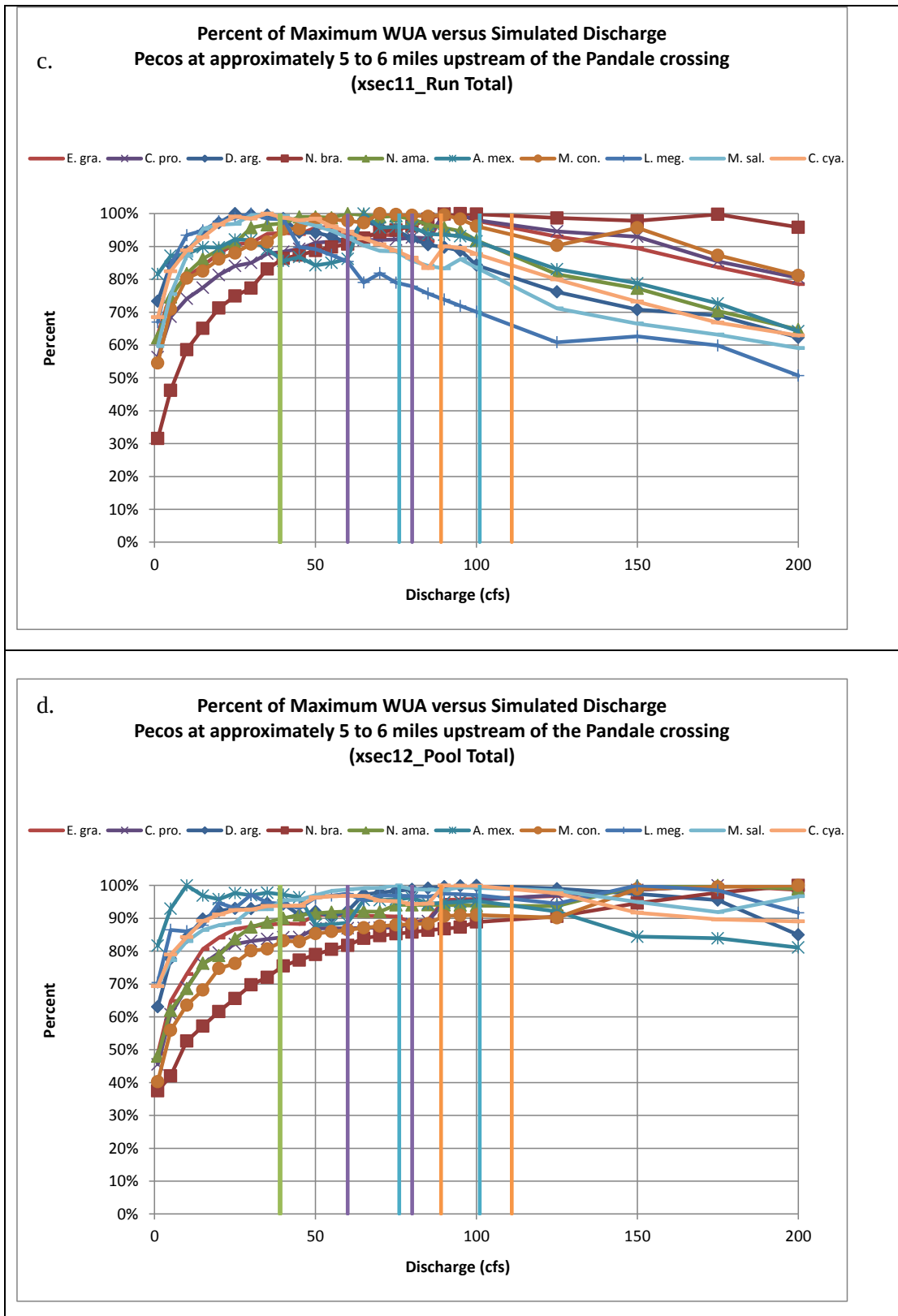
Figure 3.7-14. Percent of maximum weighted usable habitat area with a 0.5 minimum quality threshold versus modeled flow ( \text{ft}^3/\text{s} ) for 10 focal species at the Pecos River at Brotherton Ranch near Pandale. Shown are percent of maximum WUA versus flow relationships for a) all cross-sections, b) riffle cross-sections, 3) run cross-sections and d) pool cross-sections. Vertical bars bracket environmental flow regime components.
