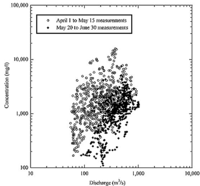
Figure 3.6-9. Plot of suspended sediment concentration vs. discharge on the Green River near Jenson, UT showing the 2 orders of magnitude difference in suspended-sediment concentration in relation to discharge. Figure taken from Grams and Schmidt (2002).
