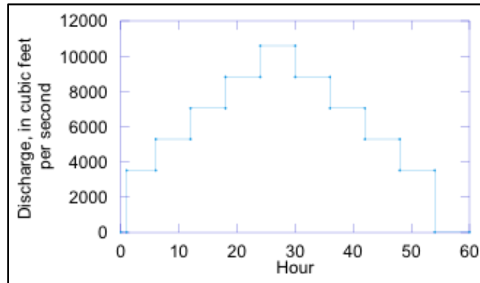
Figure 3.6-13. Stepped hydrograph used in the 1-dimensional sediment analysis completed using HEC-RAS.
