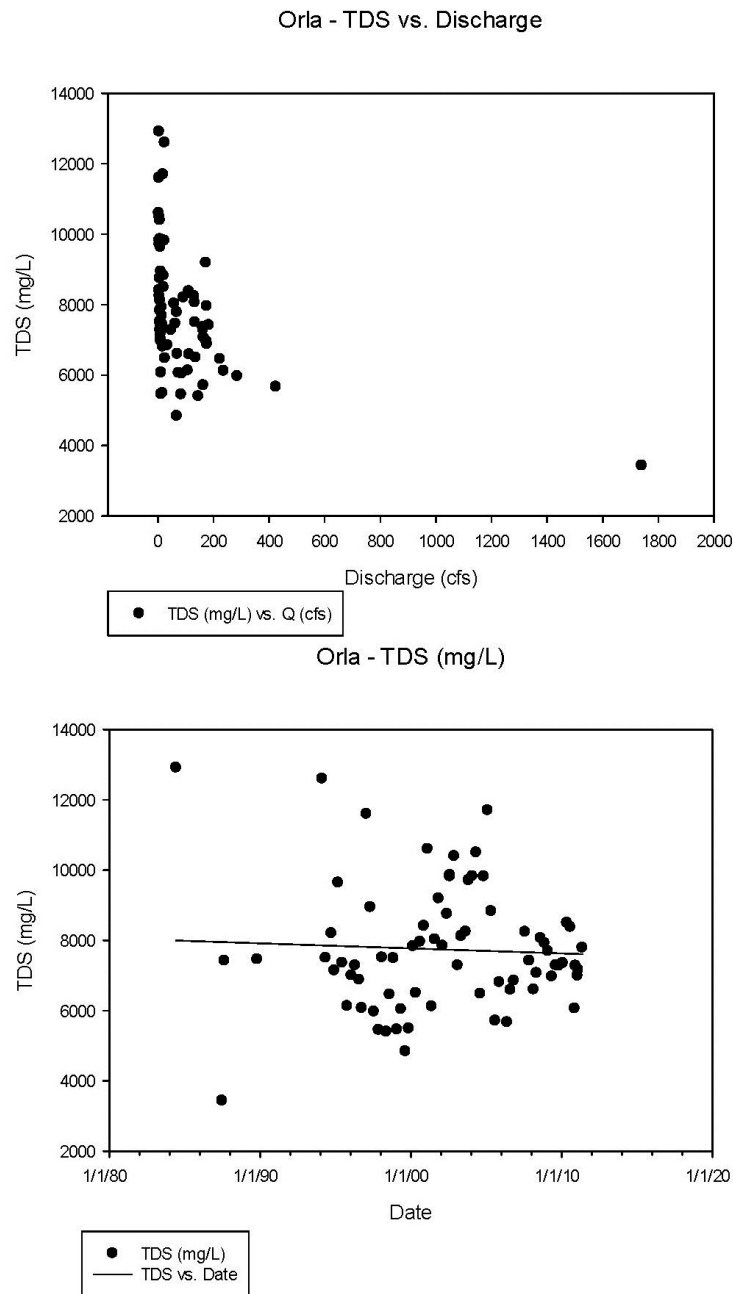
Figure 3.7-2. Water quality data for the Pecos River at Orla.
