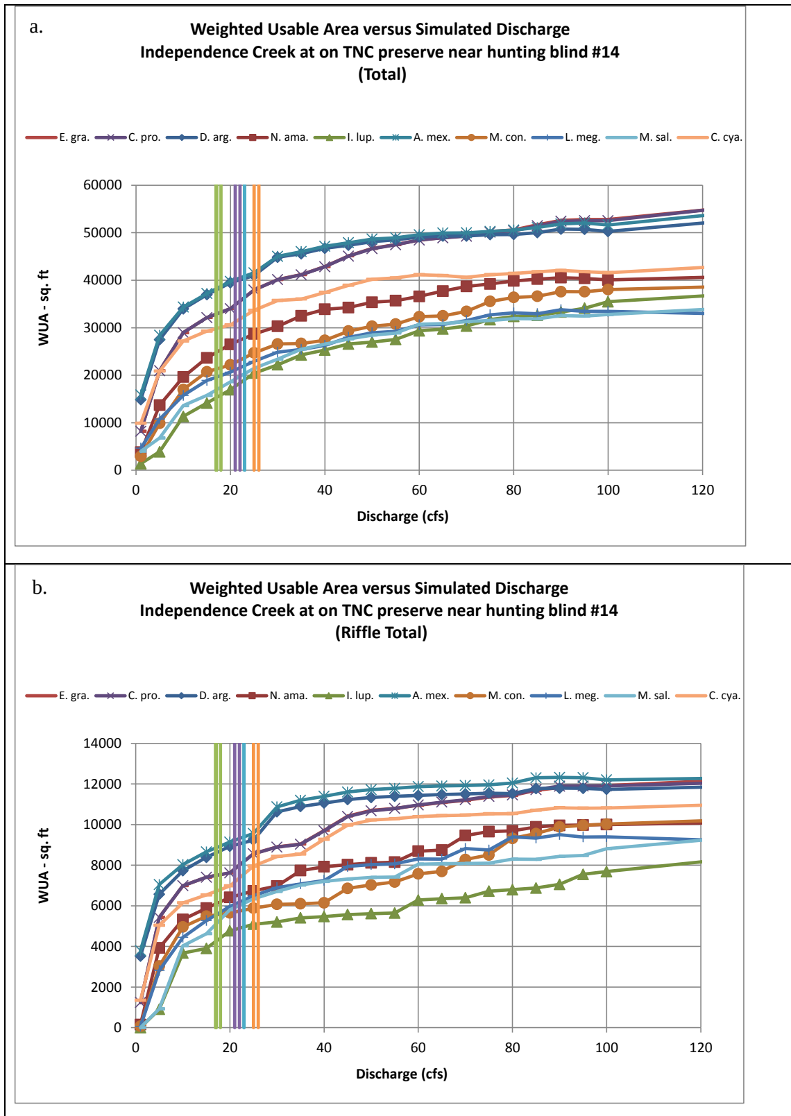
Figure 3.7-9. Weighted usable habitat area with a 0.5 minimum quality threshold versus modeled flow ( \text{ft}^3/\text{s} ) for 10 focal species at Independence Creek near Sheffield. Shown are WUA versus flow relationships for a) all cross-sections, b) riffle cross-sections, c) run cross-sections and d) pool cross-sections. Vertical bars bracket environmental flow regime components.
