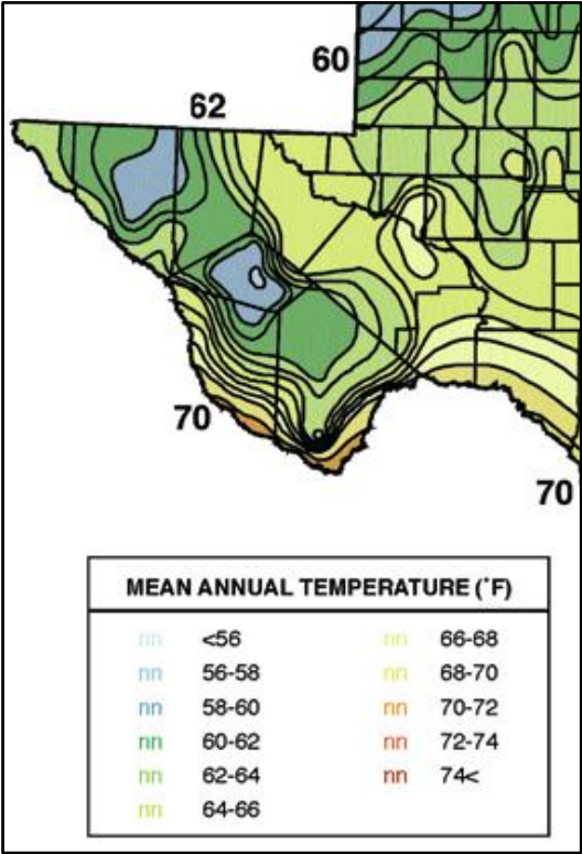
Figure 2.3-3. Average Annual Temperature (TECO, 2008).
