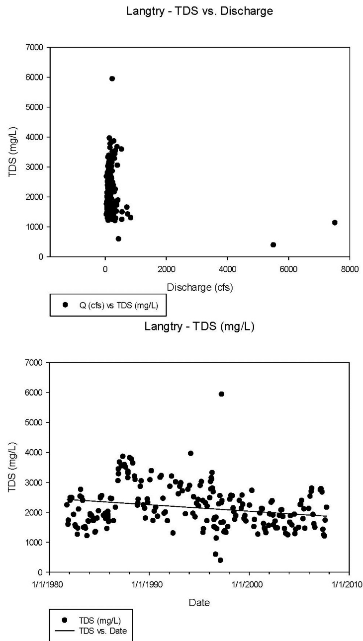
Figure 3.7-7. Water quality data from the Pecos River at Langtry.
