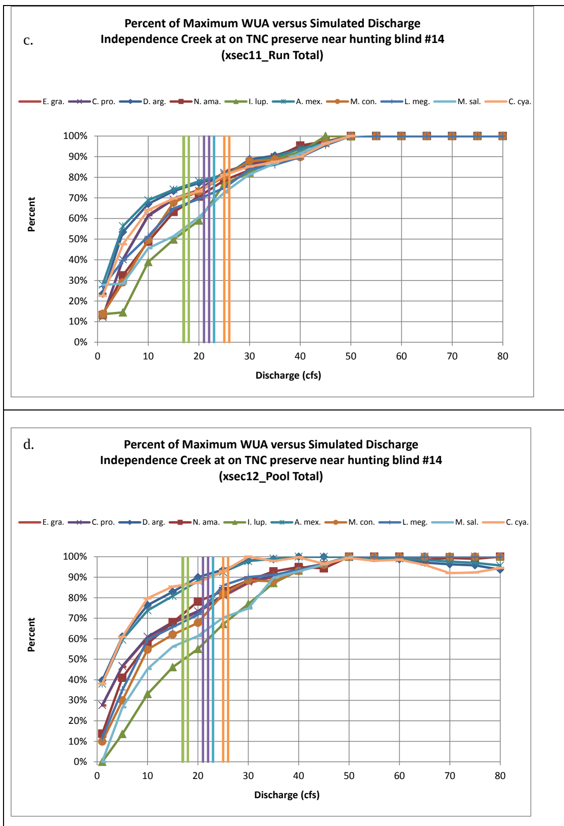
Figure 3.7-10. Percent of maximum weighted usable habitat area with a 0.5 minimum quality threshold versus modeled flow (ft 3 /s) for 10 focal species at Independence Creek near Sheffield. Shown are percent of maximum WUA versus flow relationships for a) all cross-sections, b) riffle cross-sections, 3) run cross-sections and d) pool cross-sections. Vertical bars bracket environmental flow regime components.
