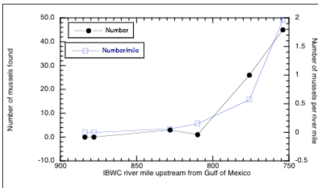
Figure 3.6-6. Results from a mussel survey conducted in 2005 depicting downstream increase in abundance. Reported river mile is at the downstream end of each sampling reach.
