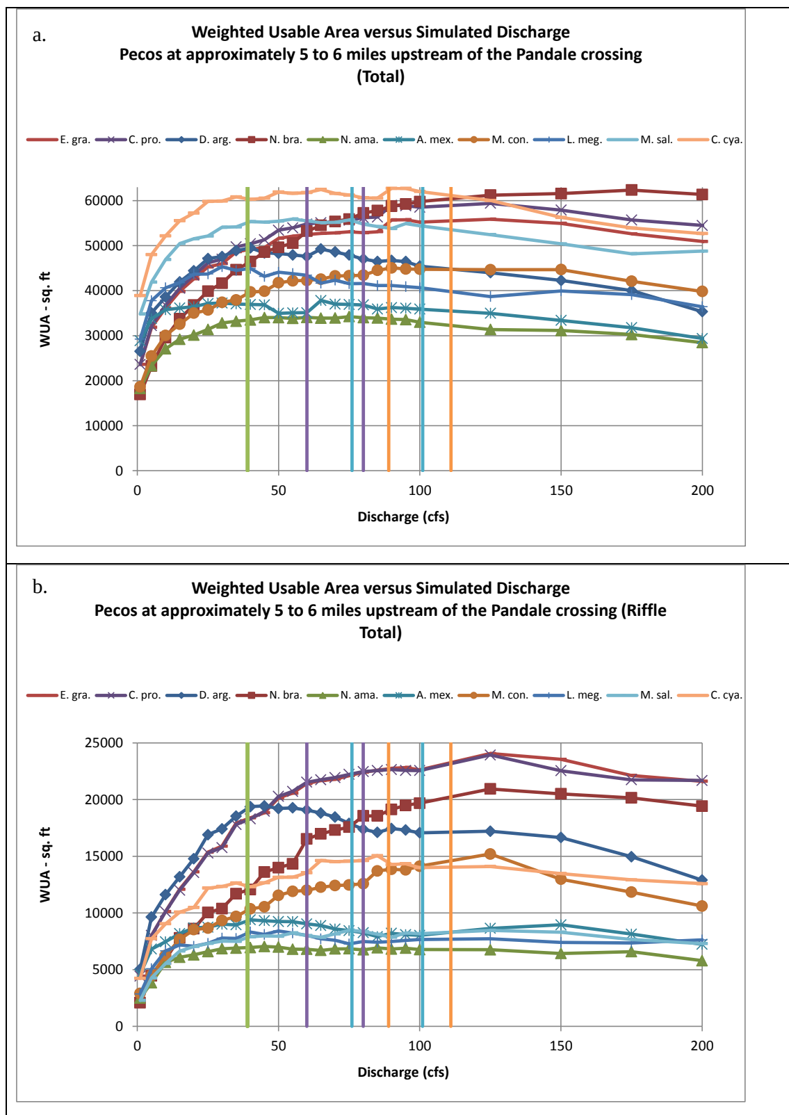
Figure 3.7-13. Weighted usable habitat area with a 0.5 minimum quality threshold versus modeled flow ( \text{ft}^3/\text{s} ) for 10 focal species at the Pecos River at Brotherton Ranch near Pandale. Shown are WUA versus flow relationships for a) all cross-sections, b) riffle cross-sections, 3) run cross-sections and d) pool cross-sections. Vertical bars bracket environmental flow regime components.
